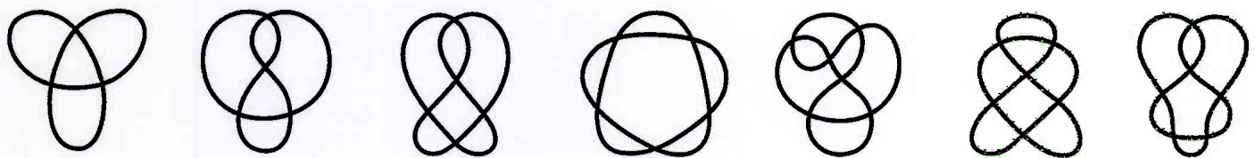
Figure 7. In an effort to develop a table of elements based on the vortex-atom theory, Tait began to classify knots according to the number of crossings. The seven simplest knots, above, extend through six crossings. Tait eventually built tables through ten-crossing knots. Current tables extend through 16 crossings and contain more than 1.7 million entries.
