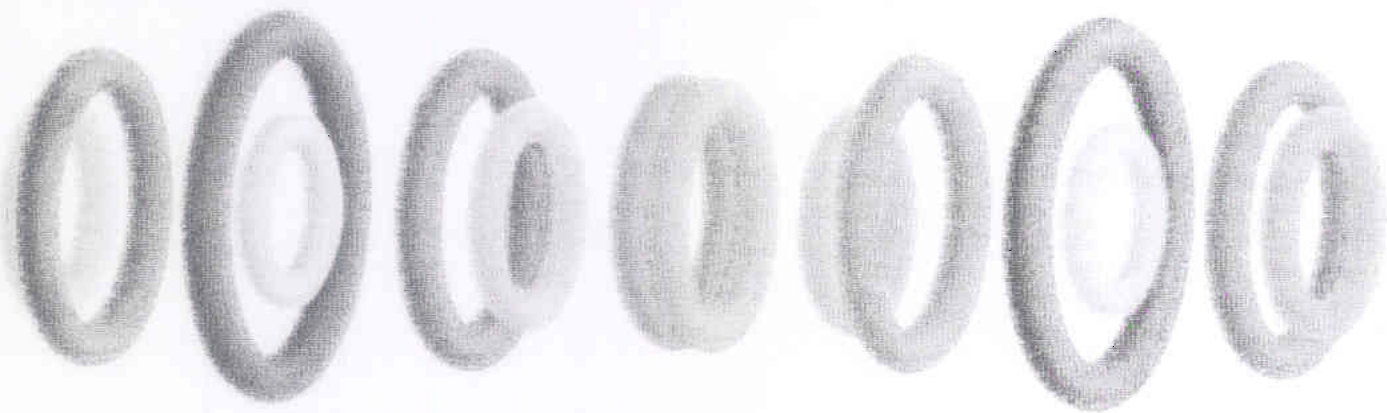
Figure 4. In a paper published in 1858, Hermann von Helmholtz described the motion of vortex rings in a perfect fluid. He concluded that if two rings (here, one blue and one green) moved in the same direction on the same plane, the first ring would enlarge and slow down, and the second ring would shrink and pass through the first ring. This process would repeat indefinitely. Tait used his smoke-ring box to illustrate Helmholtz's conclusions and found that he was able to reproduce this interaction.
