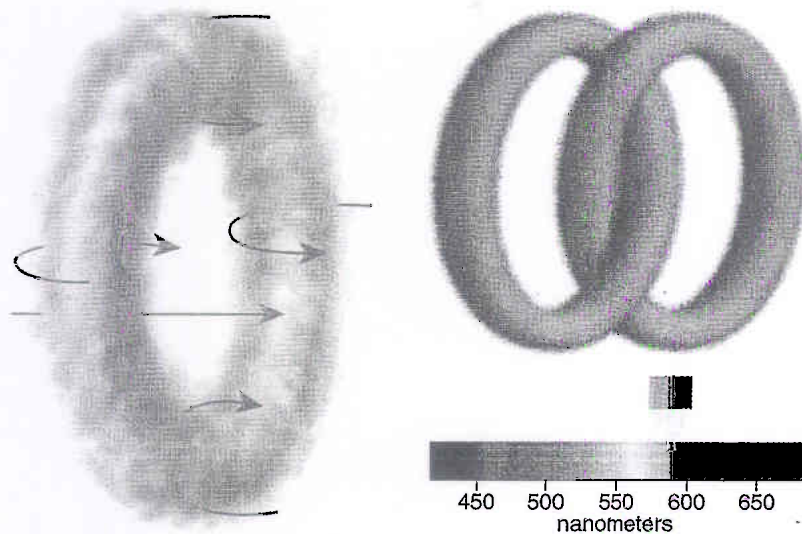
Figure 3. William Thomson’s vortex-atom theory arose out of his observations of Tait’s experiments with smoke rings. The arrows around the smoke ring at left indicate the direction of the vortex motion. Air pushes against the greater surface area of the outer part of the ring, moving the ring in the direction of the air passing through the inside of the ring. In a perfect fluid, such as the ether, this vortex motion would be permanent. Thomson posited that the behavior of atoms could be explained if they were knots of ether imparted with vortex motion. He used sodium as an example, thinking that the element’s distinct “D-lines,” or doublet of spectral emissions, might be caused by two linked rings of ether.
