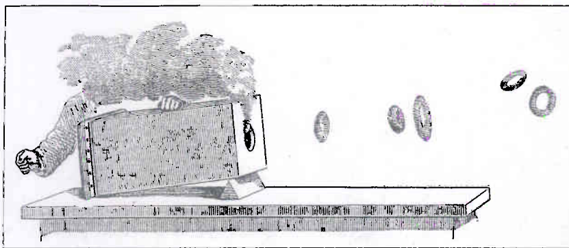
Figure 2. In 1867, Peter Guthrie Tait constructed a box to study smoke rings. He placed a towel on one end, carved a circular hole on the other end and placed ammonia and sulfuric acid inside the box. Striking the towel would cause smoke rings to emerge through the hole. As smoke reached the opening, it would move outward and then backward in a circular motion as air outside the box pushed against it. This circular pattern would create a vortex, stabilizing the smoke ring. If a shape other than a circle was used, the rings would gradually take on a circular shape after passing through the hole. This sketch of the smoke-ring box comes from Tait’s book Recent Advances in Physical Science .
